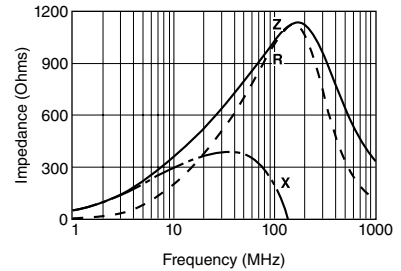
BLM11A221S
