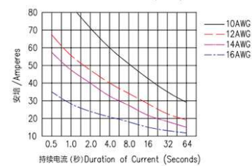
PA45多极/PA45 Multipole 脉冲电流/ Pulse Current Capability
