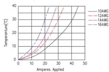
PA45单极/PA45 Singlepole 温升曲线 Temperature Rise at Constant Current
