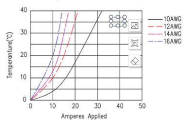
PA45多极/PA45 Multipole 温升曲线 Temperature Rise at Constant Current
