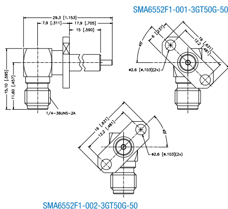
SMA6552F1-002-3GT50G-50
