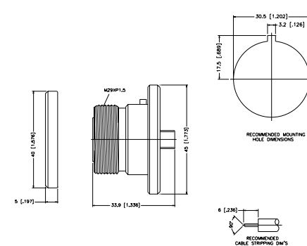
Assembly Instruction E - page 231
