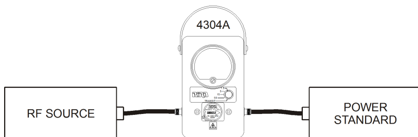
Figure 10 Calibrating the 4304A Element
