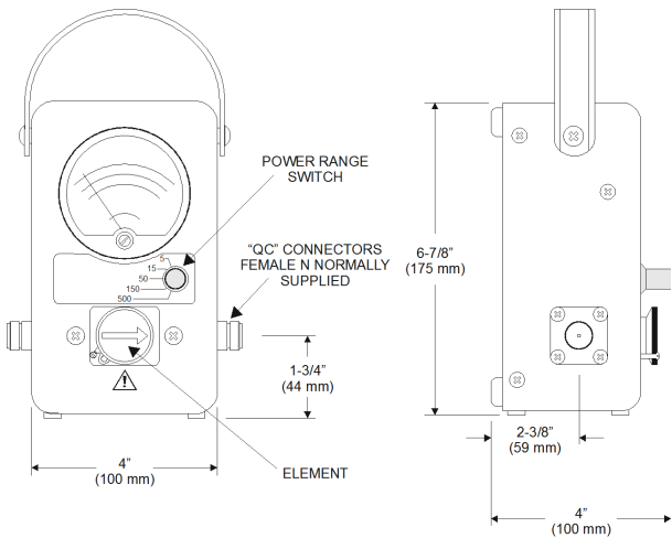
Figure 1 Bird 4304A ThruLine Wattmeter Outline Drawing
