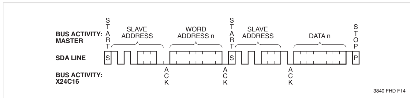
Figure 8. Random Read
