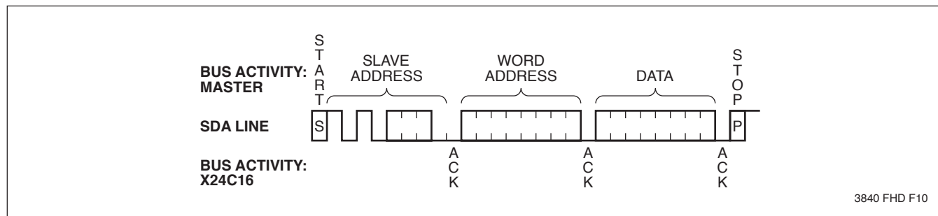
Figure 5. Byte Write
