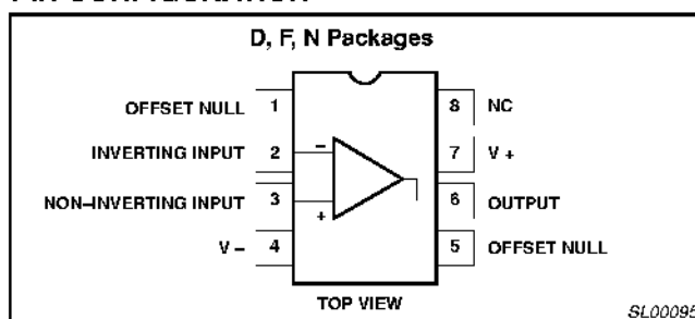
Figure 1. Pin Configuration
