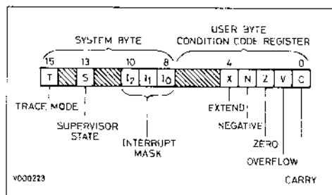
Figure 1.3 : Status Register.
