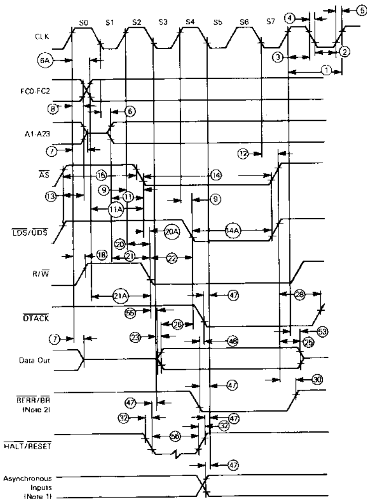
Figure 8.8 : Write Cycle Timing Diagram.
