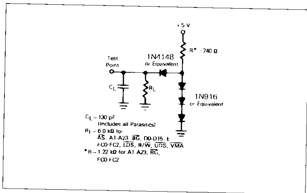
Figure 8.3 : Test Loads.
