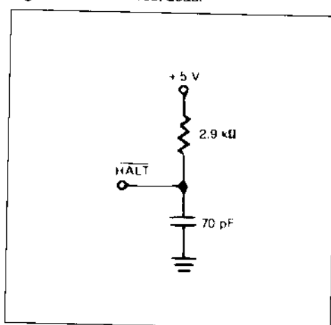
Figure 8.2 : \overline{\text{HALT}} Test Load.
