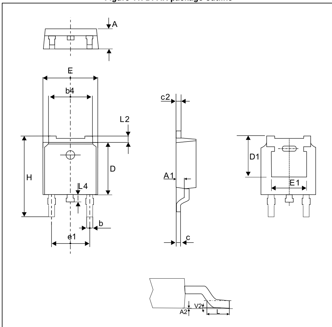
Figure 11. DPAK package outline
