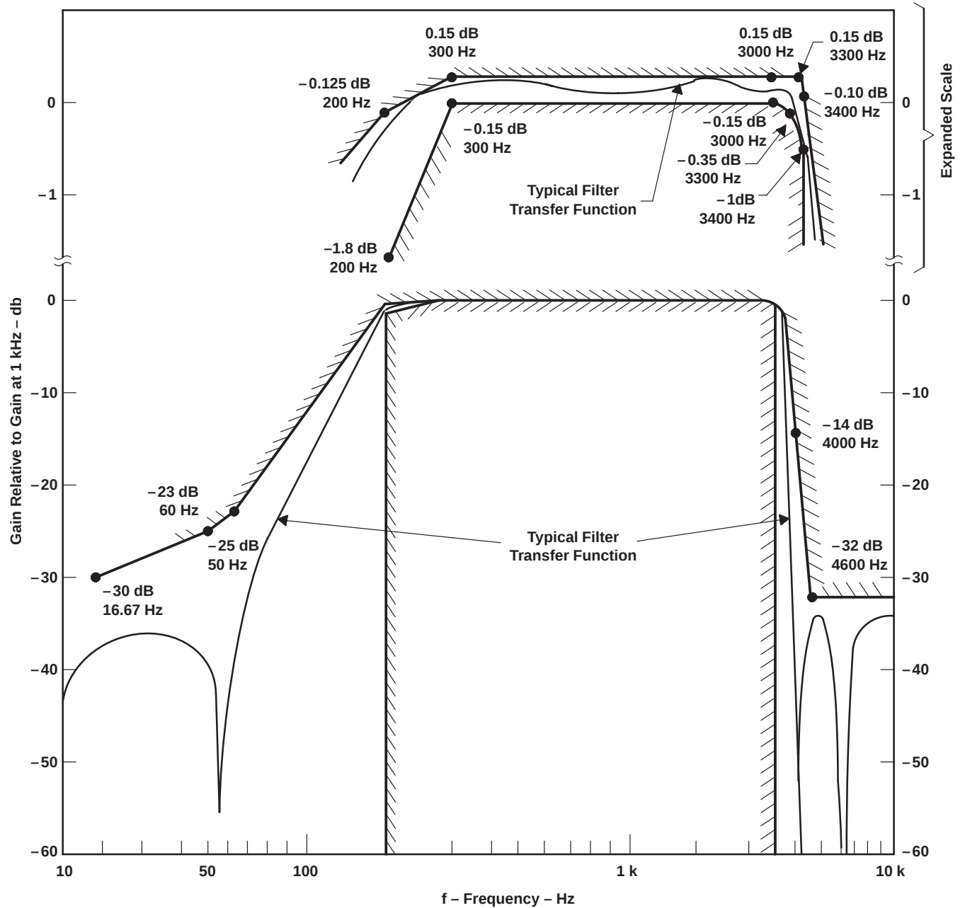
Figure 1. Transmit Filter Transfer Characteristics
