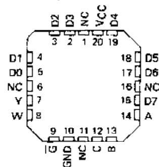
SN54LS151, SN54S151 . . . FK PACKAGE
