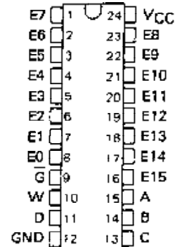
SN54151A, SN54LS151, SN54S151 . . . J OR W PACKAGE SN74151A . . . N PACKAGE
