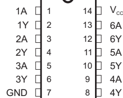
SN54HC04...J OR W PACKAGE SN74HC04...D, DB, N, NS, OR PW PACKAGE (TOP VIEW)
