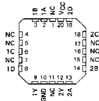
SN54LS20, SN54S20 . . . FK PACKAGE (TOP VIEW)
