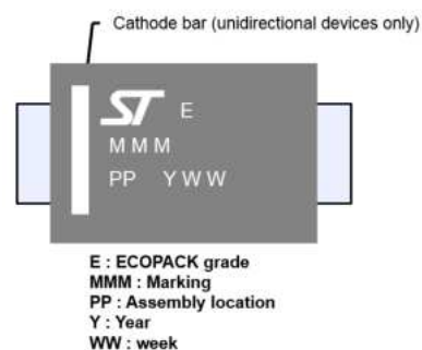
Figure 15. SMA marking
