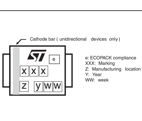
Figure 14. Marking layout (1)
