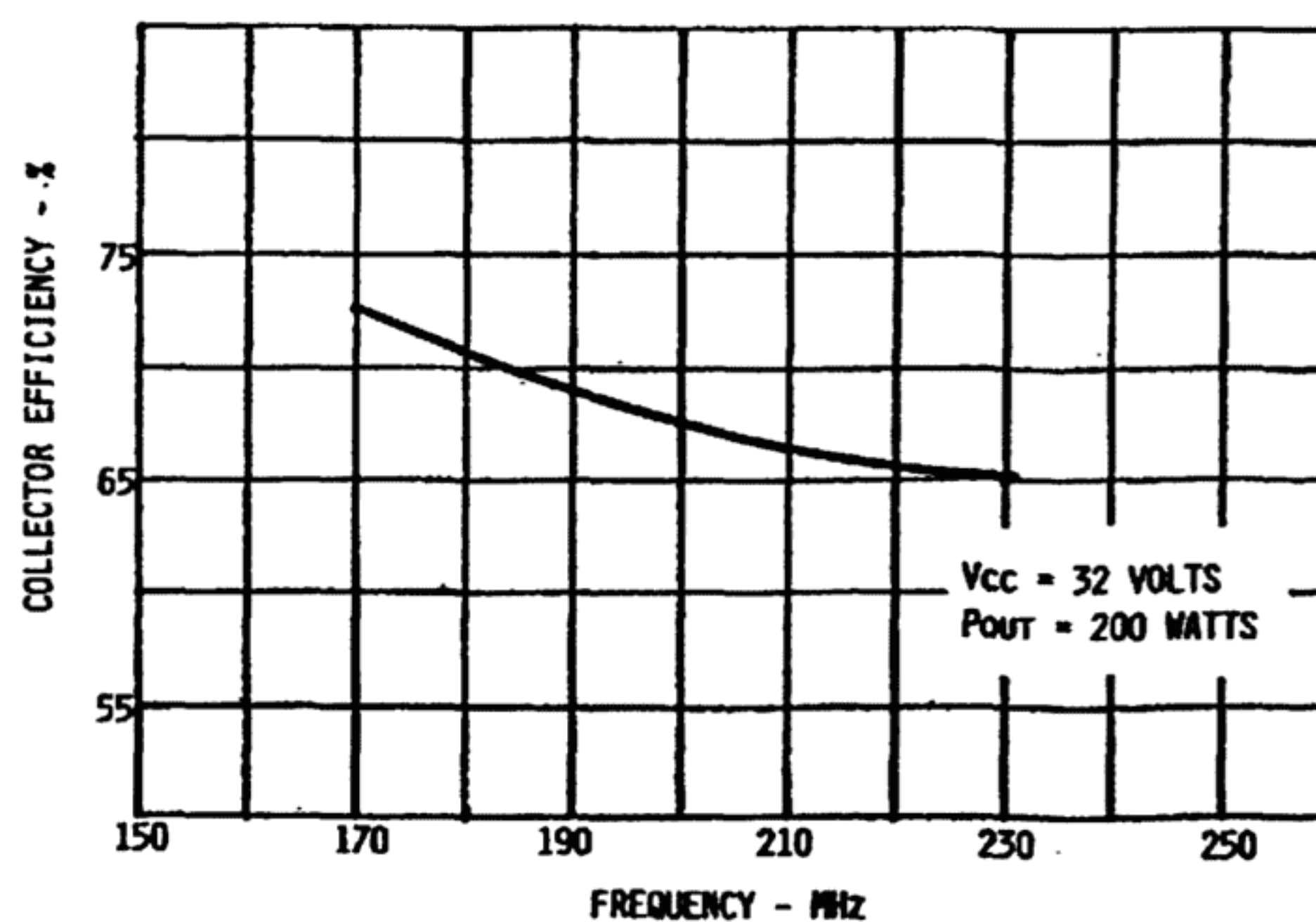
EFFICIENCY VS FREQUENCY
