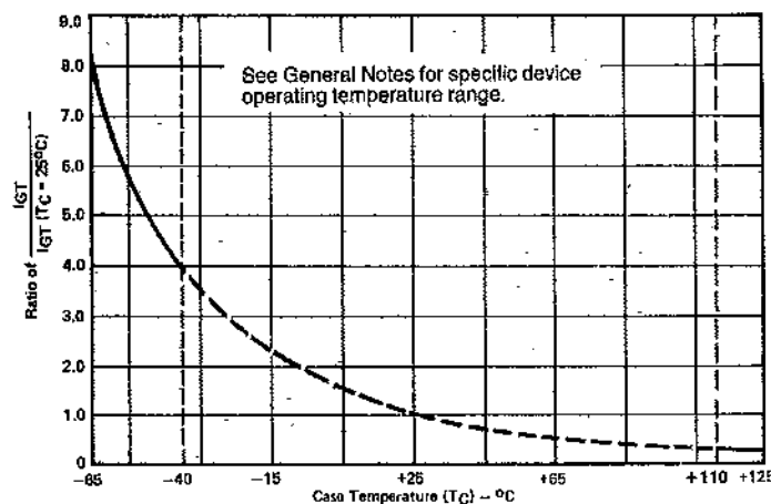
FIGURE 6 — Normalized DC Gate-Trigger Current vs Case Temperature
