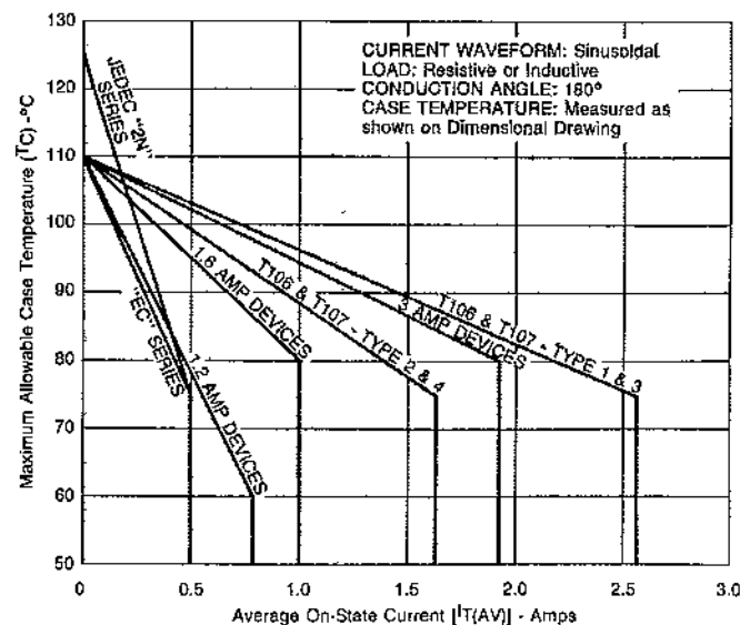
FIGURE 2 — Maximum Allowable Case Temperature vs Average On-State Current
