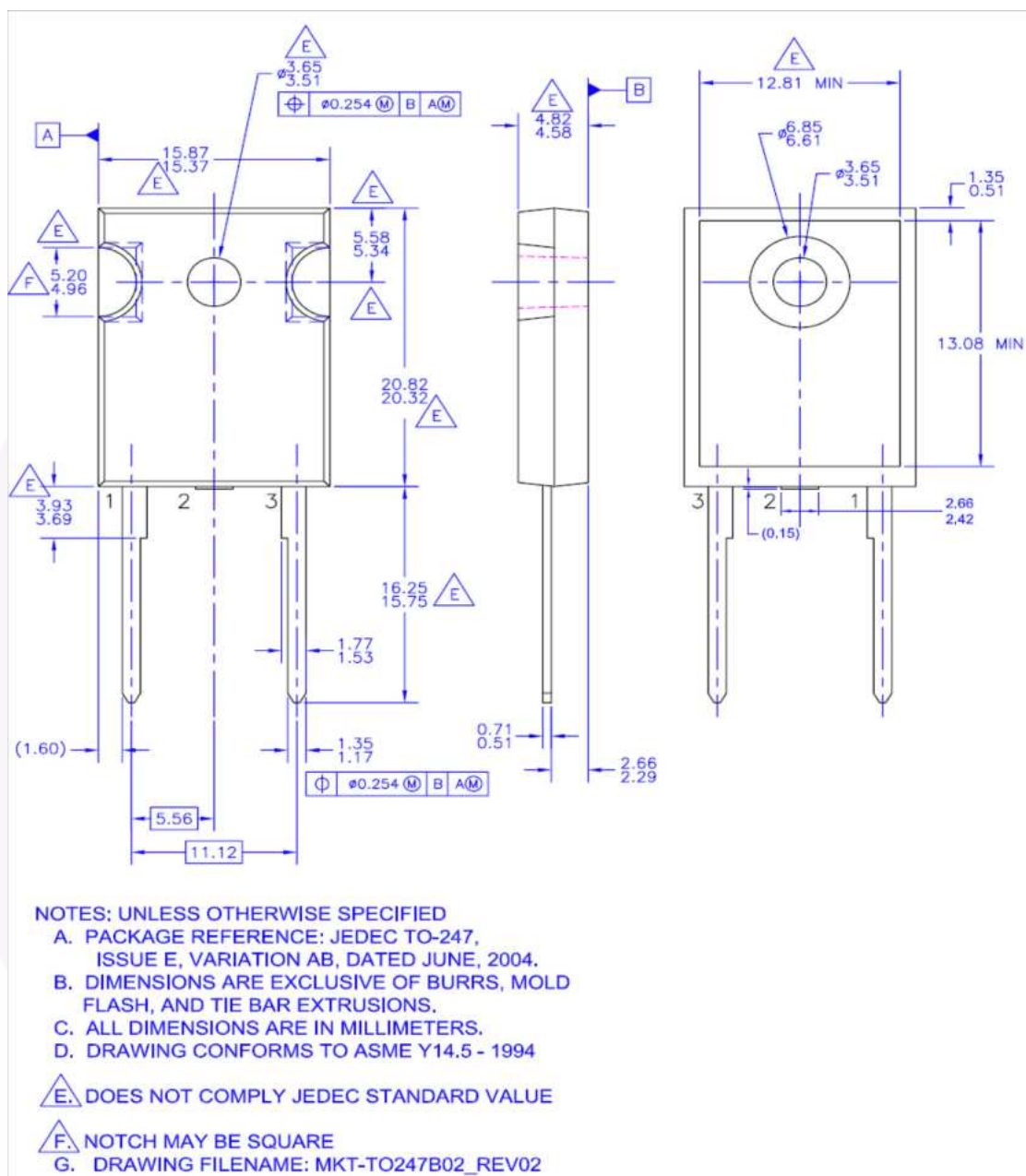
Figure 12. TO-247,Molded, 2LD, Jedec Option AB
