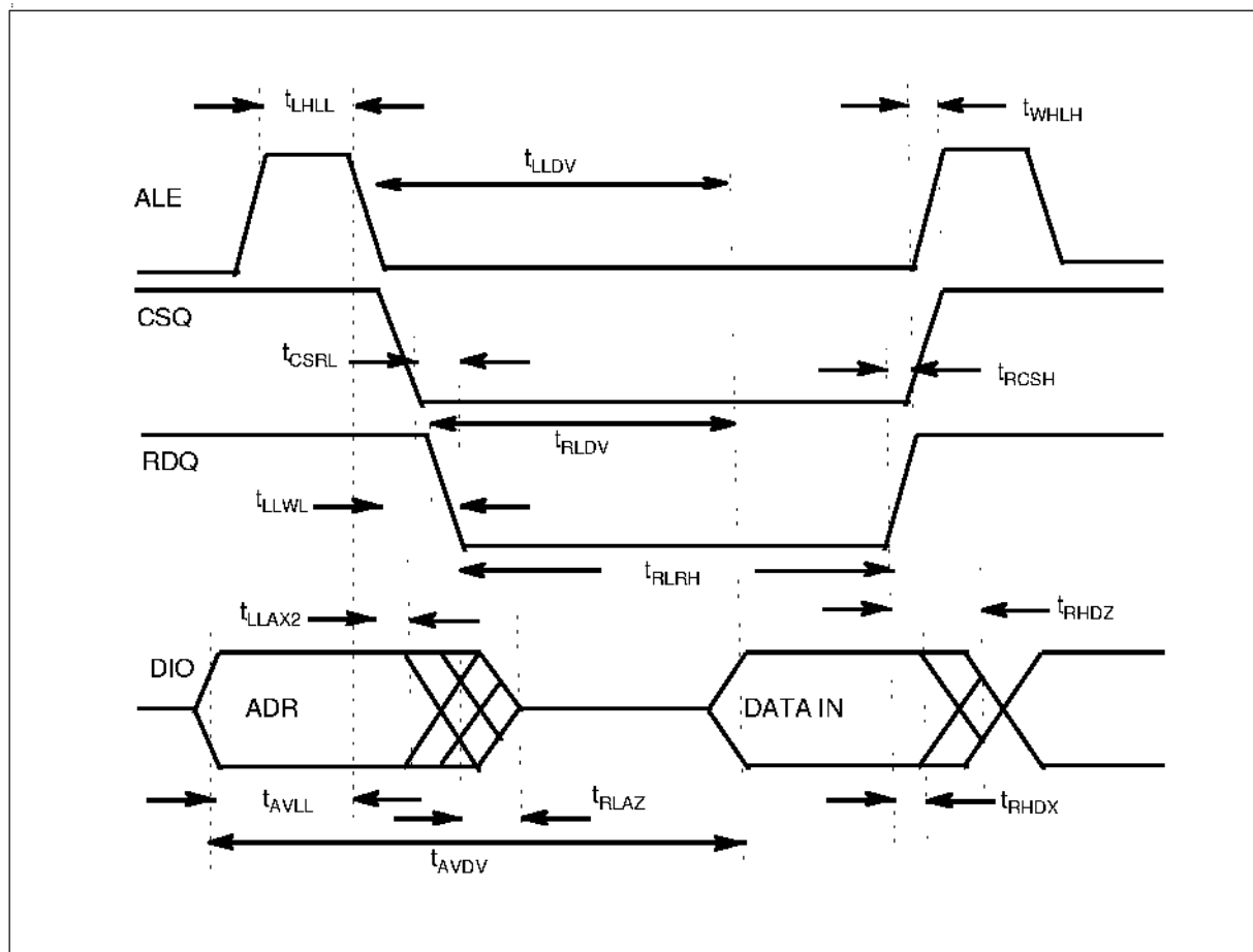
Figure 40 Timing Specifications for a Read Access to the \mu C-Interface
