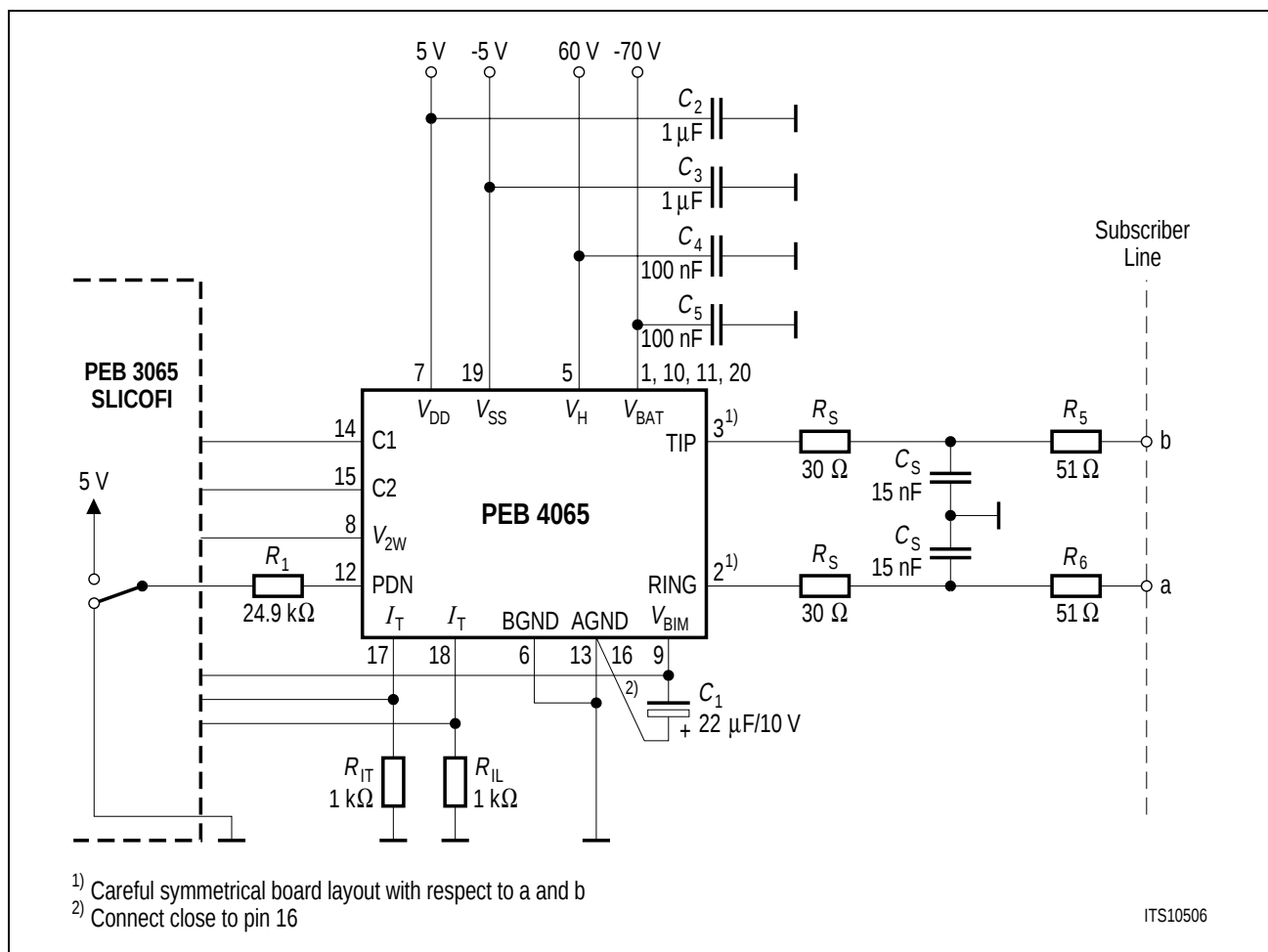
Figure 5 Application Circuit
