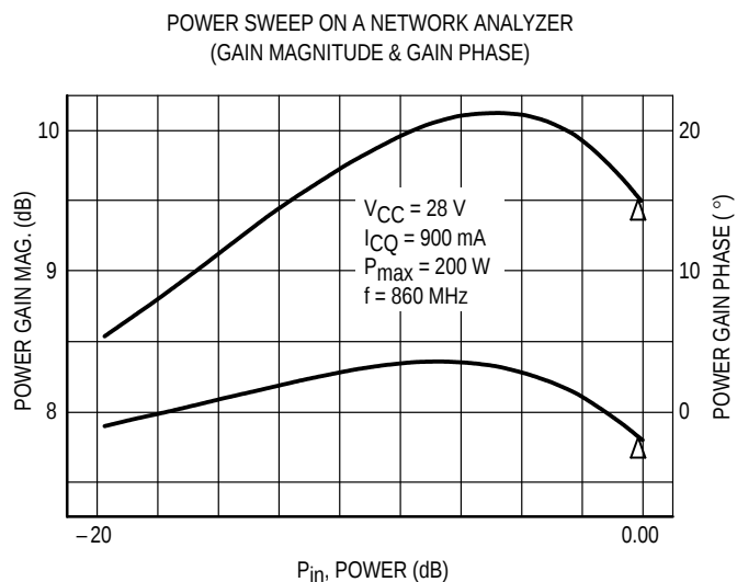
Figure 19. Power Gain versus Input Power
