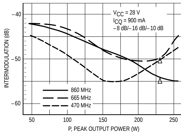
Figure 21. Intermodulation versus Output Power
