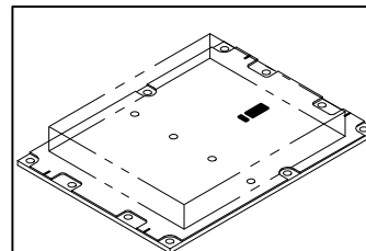
CASE 439-01, STYLE 1
