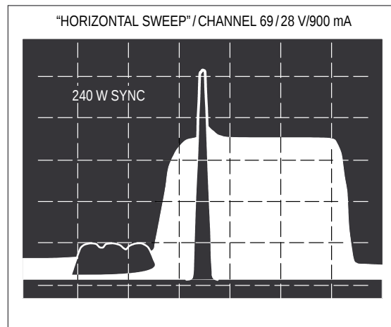
Figure 17. "Horizontal Sweep" 240 W Sync
