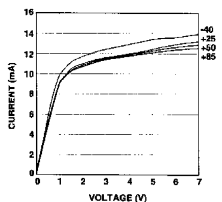
Figure 9. Device Current vs. Voltage.
