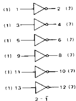
MC1820 High Voltage Hex Inverter (Without Output Resistors)
