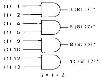
MC1806/MC1906 MC1807/MC1907 Quad 2-Input AND Gate
