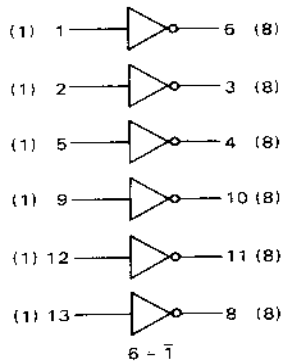
MC840/MC940 Hex Inverter (Without Input Diodes)
