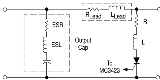
Figure 18. Circuit Elements Affecting SCR Surge &amp; di/dt
