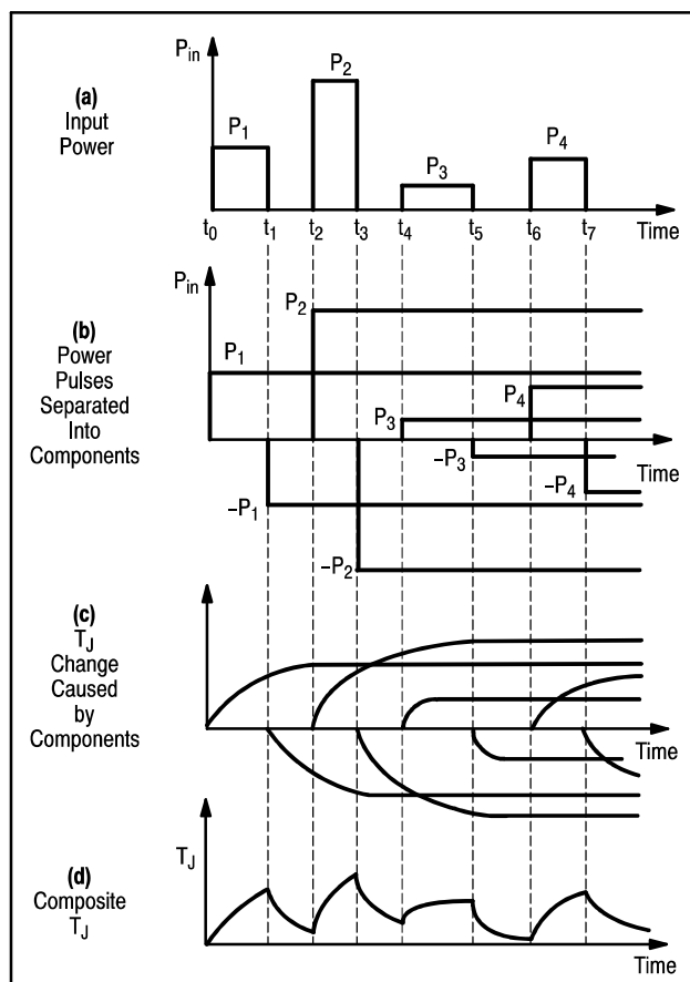
Figure 41. Application of Superposition Principle
