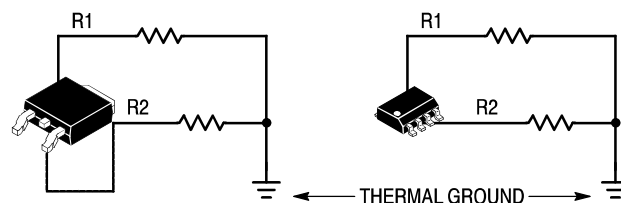
Figure 15. Parallel Resistor Analogy for Case-Mounted and Lead-Mounted Configurations
