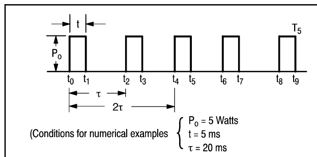
Figure 43. A Train of Equal Repetitive Pulses
