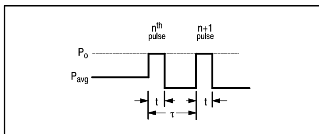
Figure 44. Model For a Repetitive Equal Pulse Train
