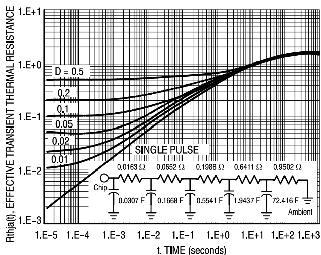
Figure 20. Transient Thermal response for MMSF5N03HD mounted on 1 in. sq. Cu area PCB.
