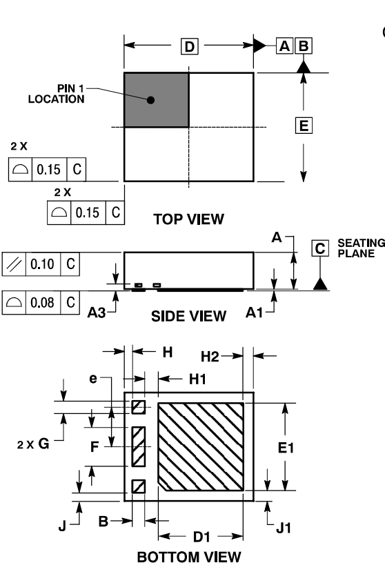
PLLP-4 CASE 508AA-01 ISSUE O
