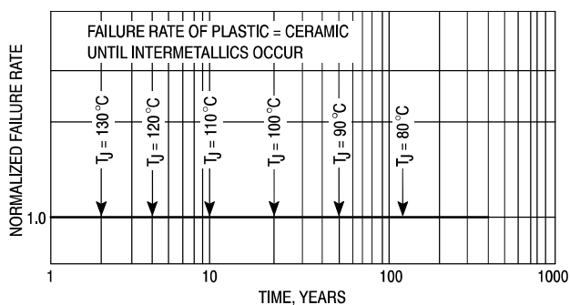
Figure 12. Failure Rate versus Time Junction Temperature
