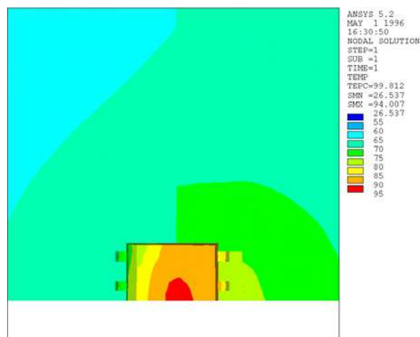
Figure 24. FEA steady-state temperature distribution on Device 1, half symmetry model at 0.96 W.
