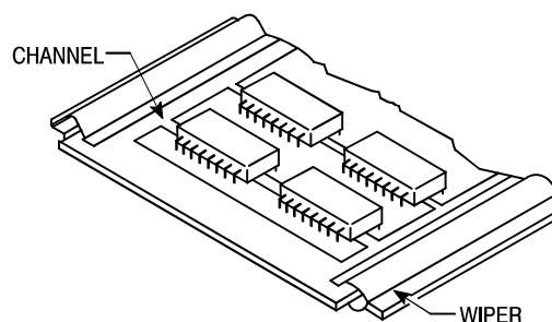
Figure 13. Channel/Wiper Heatsinking on Double Layer Board
