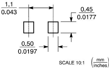
SOLDERING FOOTPRINT
