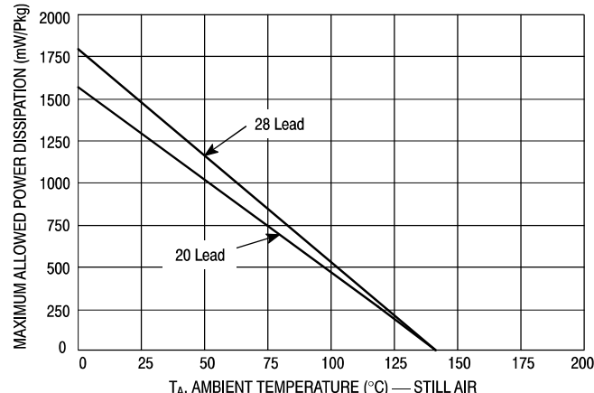
Figure 8. Ambient Temperature Derating Curves (PLCC Pkg)
