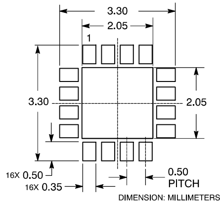
MOUNTING FOOTPRINT
