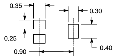
SOLDERING FOOTPRINT
