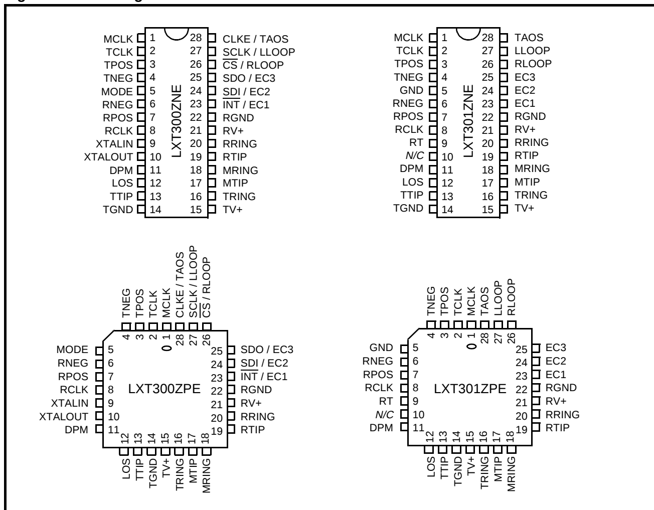
Figure 1: Pin Assignments
