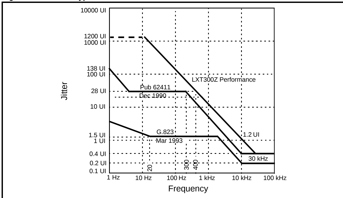
Figure 10: LXT300Z Typical Receive Jitter Transfer Performance
