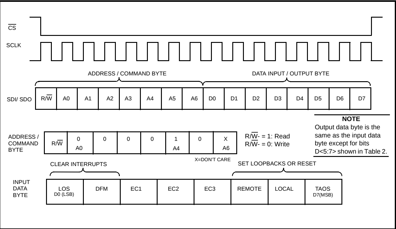
Figure 4: LXT300Z Serial Interface Data Structure
