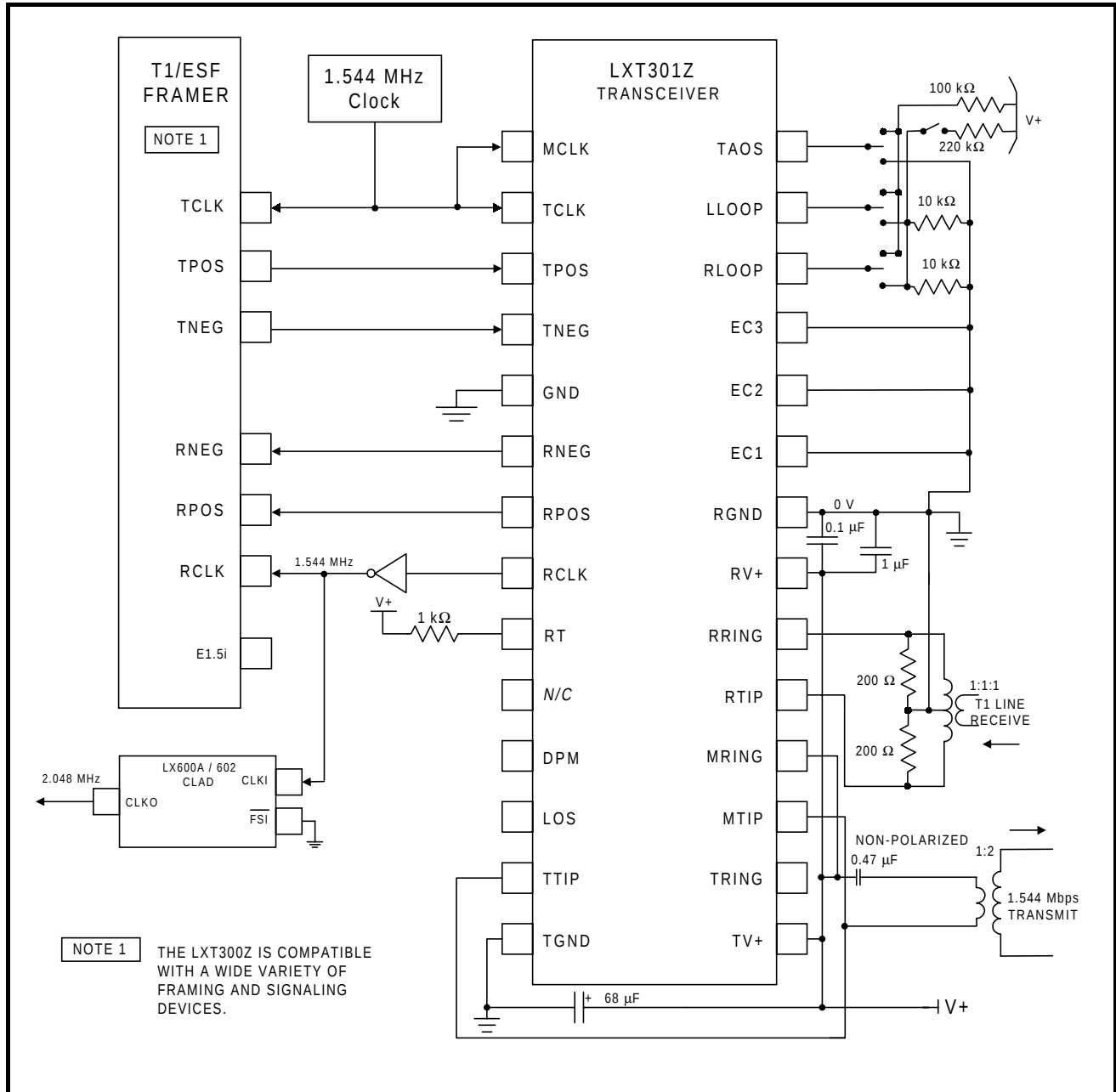
Figure 7: Typical LXT301Z 1.544 Mbps T1 Application
