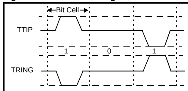
Figure 3: 50% AMI Coding
