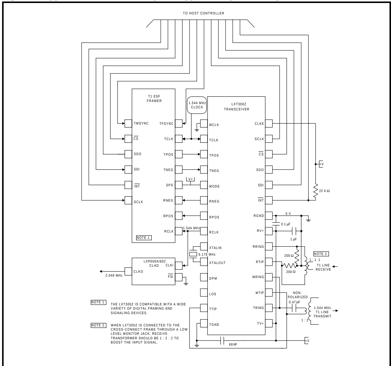
Figure 5: Typical LXT300Z 1.544 Mbps T1 Application (Host Mode)
