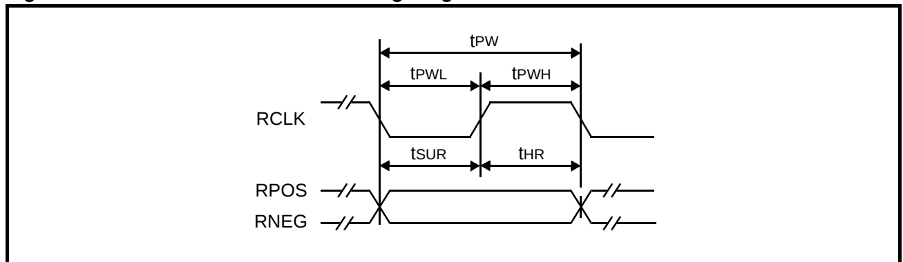
Figure 12: LXT301Z Receive Clock Timing Diagram
