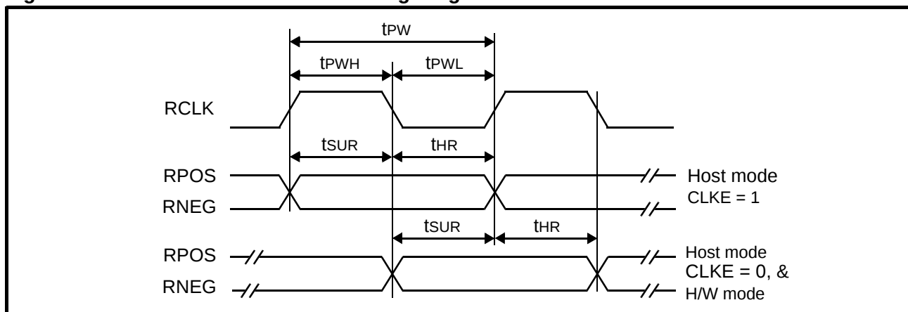
Figure 11: LXT300Z Receive Clock Timing Diagram
