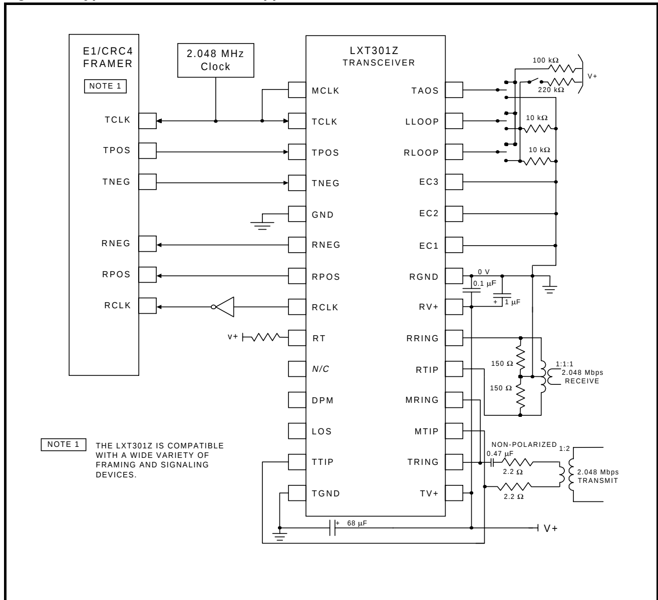
Figure 8: Typical LXT301Z 75 \Omega E1 Application
