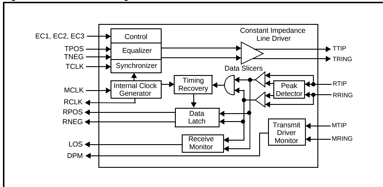
Figure 2: LXT301Z Block Diagram
