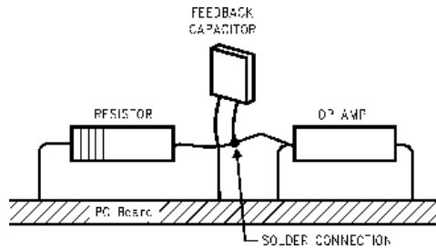
Figure 21. Air Wiring
