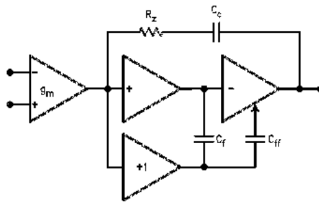
Figure 15. LMC660 Circuit Topology (Each Amplifier)
