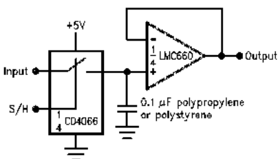
Figure 23. Low-Leakage Sample-and-Hold
