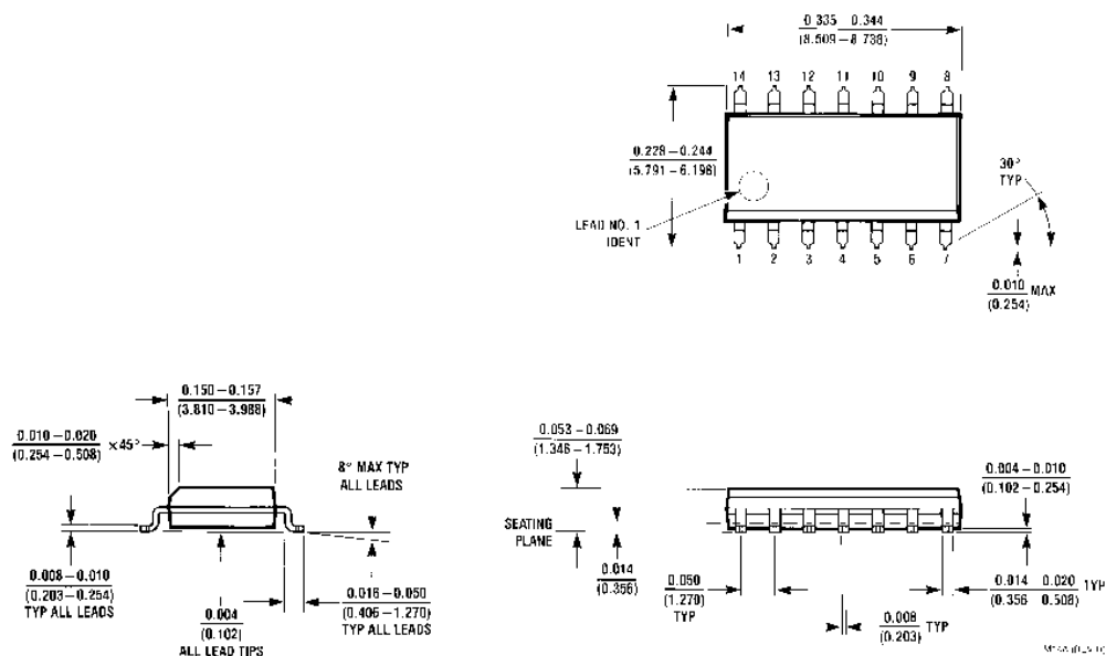
14-Pin Small Outline Order Package Number LMC6484AIM or LMC6484IM NS Package Number M14A
