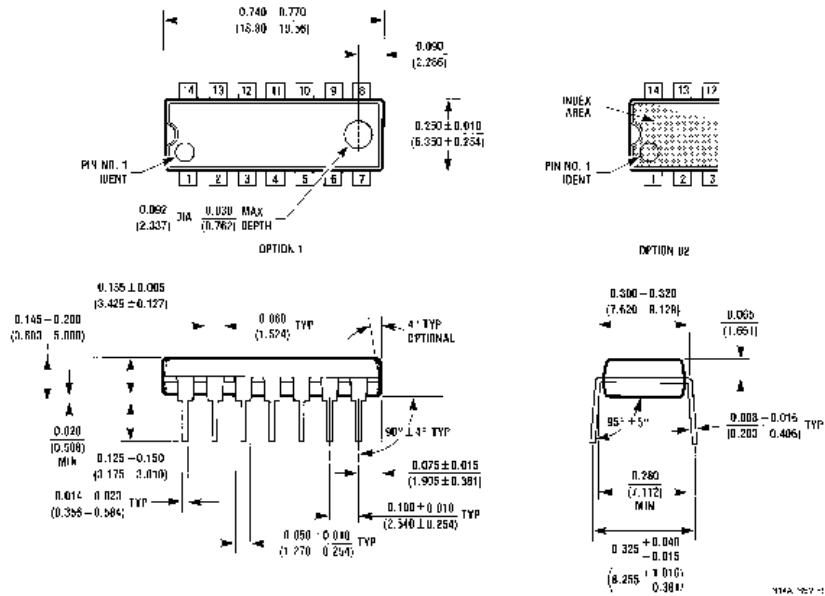
14-Pin Molded DIP
