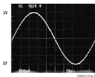
Rail-to-Rail Input
