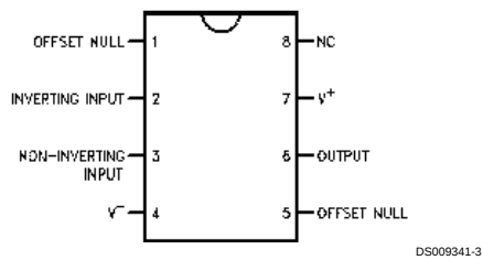
Dual-In-Line or S.O. Package
