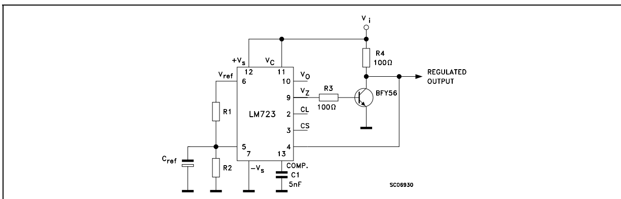
Figure 23 : Shunt Regulator
