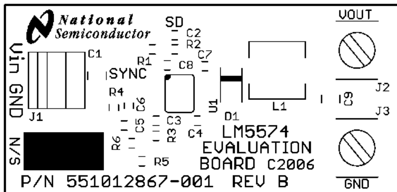
Figure 24. Silkscreen
