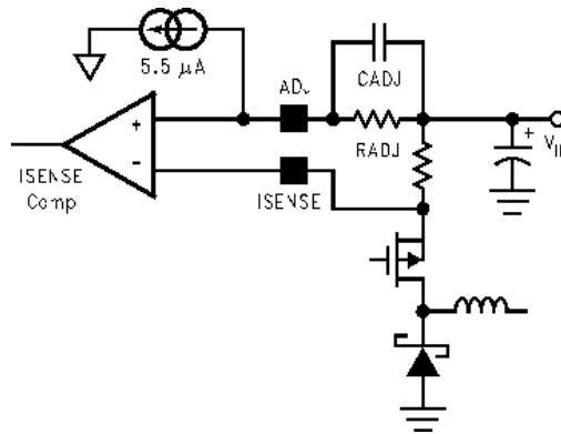
Figure 6. Current Sensing by External Resistor
