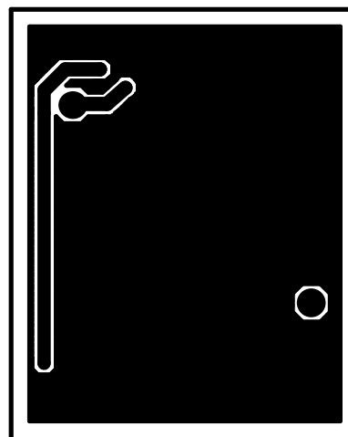
Figure 9. Bottom Layer, Typical PCB Layout (3.3V Output)
