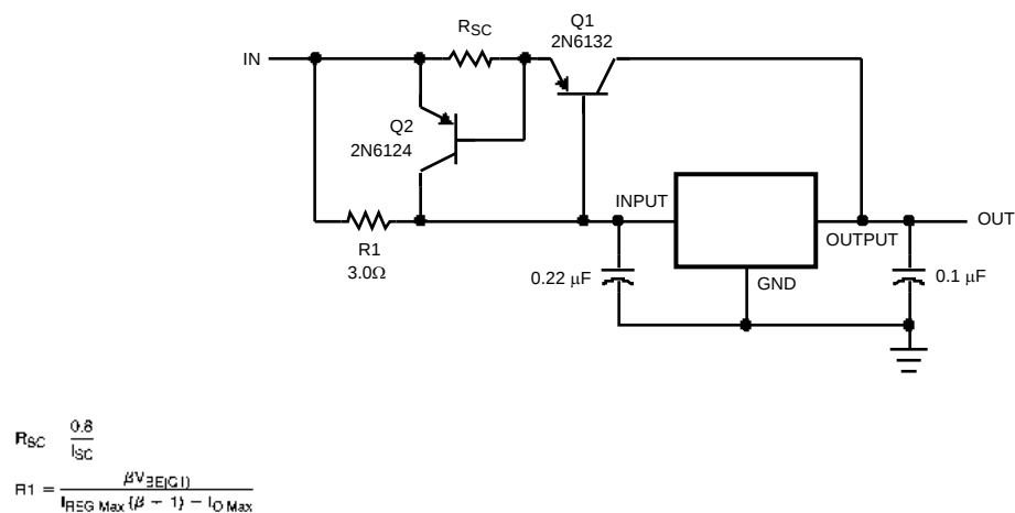
Figure 31. High Output Current, Short Circuit Protected
