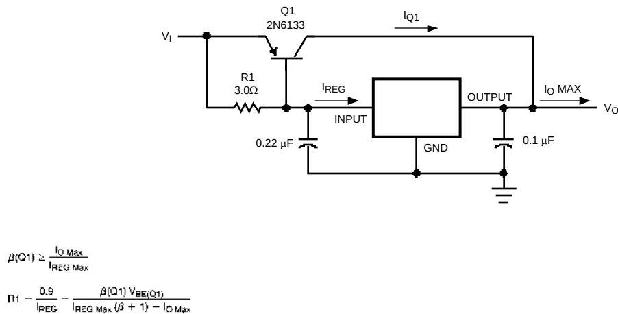
Figure 30. High Current Voltage Regulator
