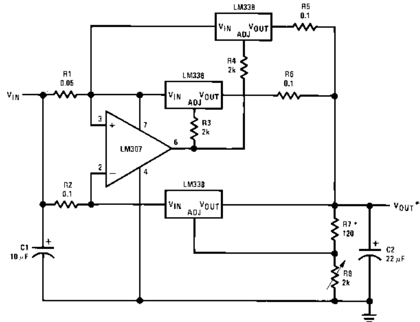
15A Regulator
