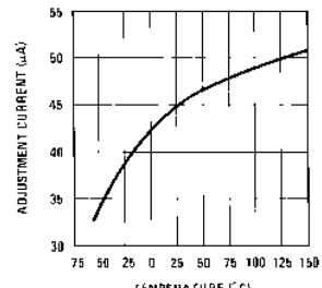
Adjustment Current
