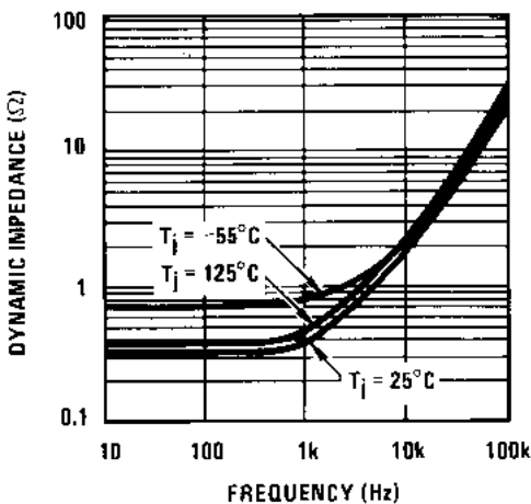
Figure 5. Dynamic Impedance
