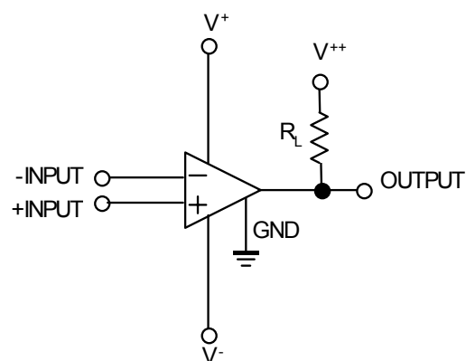
Dual Supply
