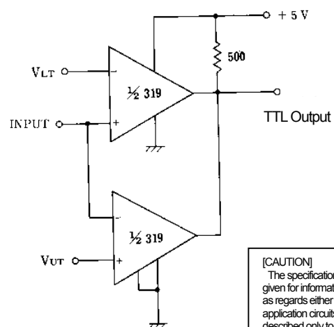
Window Detector
