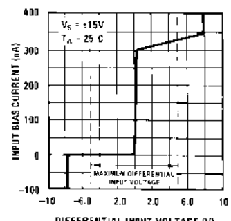
Figure 6. Input Characteristics
