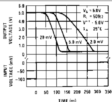
Figure 19. Response Time for Various Input Overdrives
