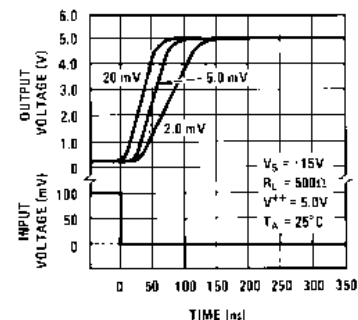
Figure 5. Response Time for Various Input Overdrives
