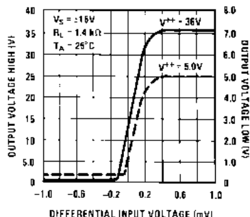
Figure 3. Transfer Function
