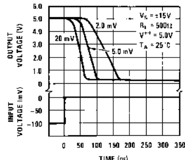
Figure 4. Response Time for Various Input Overdrives
