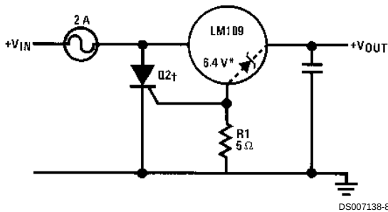
Input Crowbar
