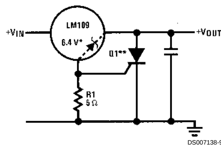
Output Crowbar
