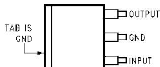
TO-263 (S) Surface-Mount Package
