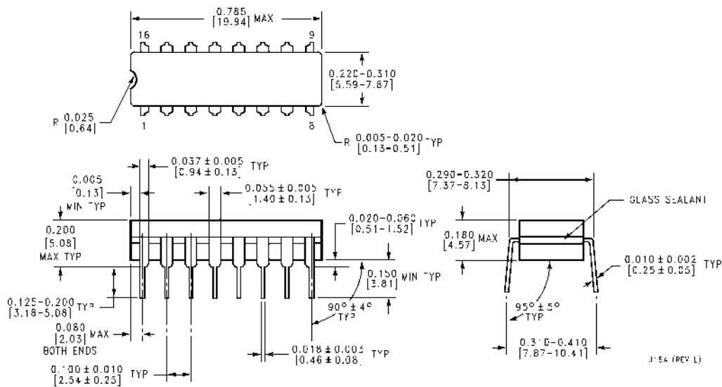
16 Lead Dual-in-Line Package (J) See NS Package Number J16A
