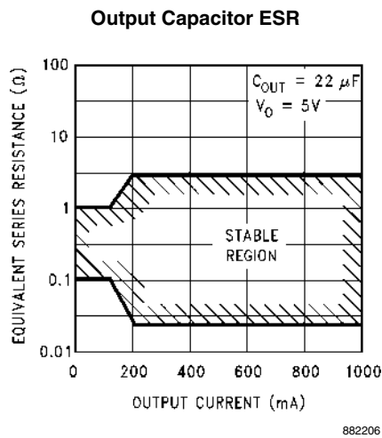
FIGURE 1. ESR Limits
