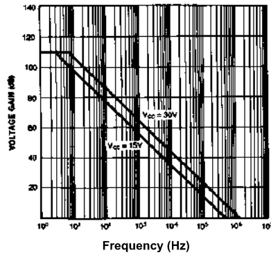
Figure 5. Open Loop Frequency Response
