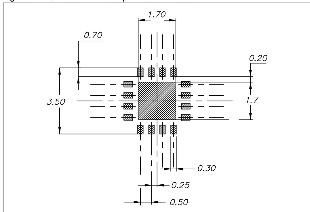
Figure 24. QFN16 3 x 3 mm footprint recommendation
