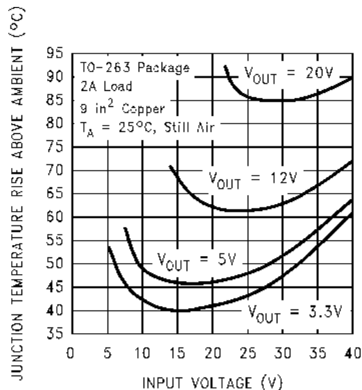
Figure 36. Junction Temperature Rise, DDPAK
