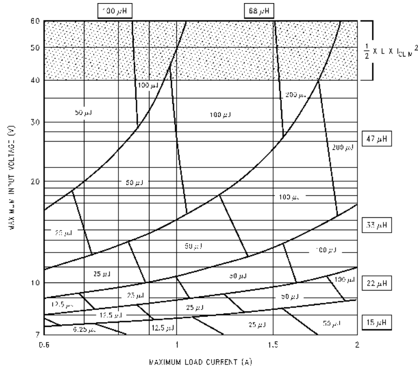
Figure 26. LM2592HV-5.0
