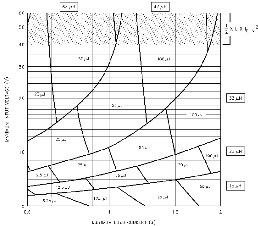
Figure 25. LM2592HV-3.3
