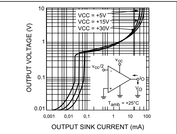
Figure 7. Output characteristics
