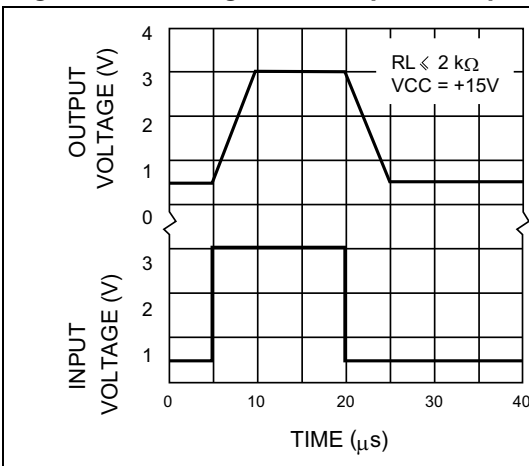
Figure 4. Voltage follower pulse response
