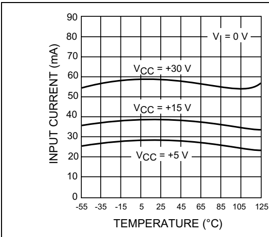
Figure 6. Input current
