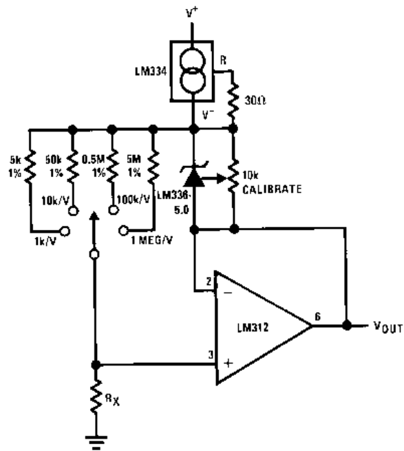
Linear Ohmmeter
