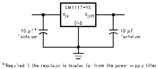
Figure 16. Fixed Output Regulator
