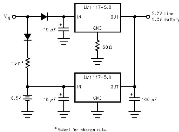
Figure 20. Battery Backed-Up Regulated Supply
