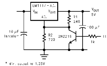
Figure 19. 5-V Logic Regulator With Electronic Shutdown*
