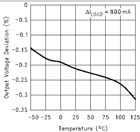
Figure 3. Load Regulation
