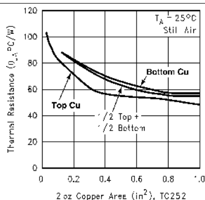
Figure 25. R_{\theta JA} vs 2-oz Copper Area for TO-252
