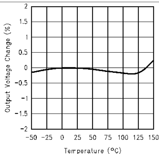
Figure 6. Temperature Stability
