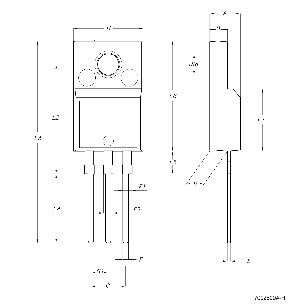
Figure 39. TO-220FP drawing
