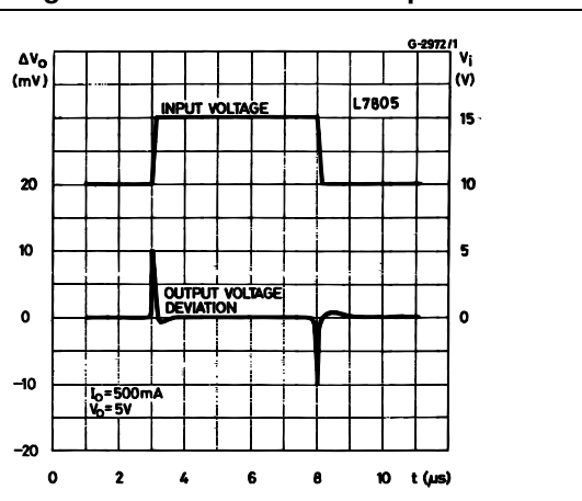
Figure 35. Line transient response
