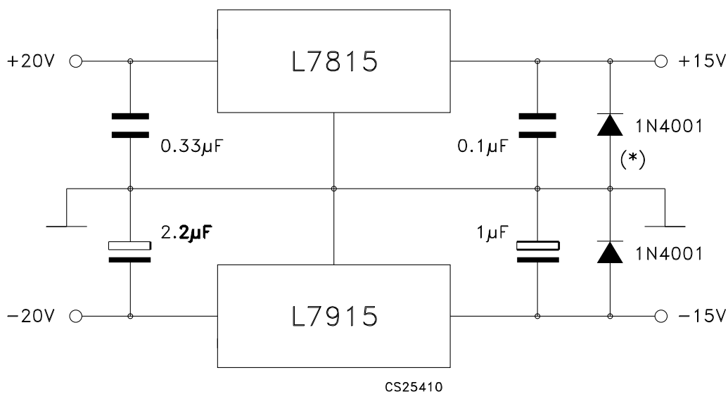
Figure 16. Split power supply ( \pm 15 V - 1 A )
