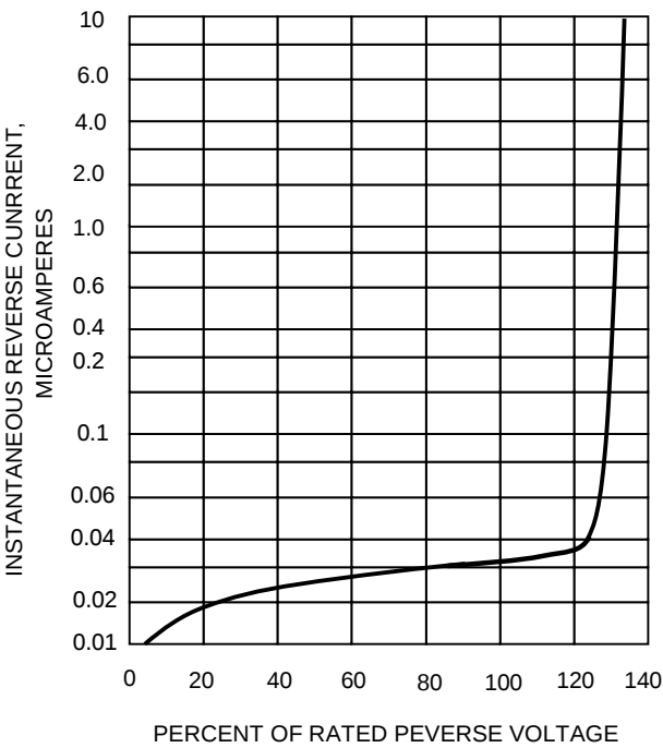
FIG.4-TYPICAL REVERSE CHARACTERISTICS
