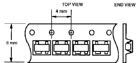
Figure 18. Option L31 for SOT-143 Packages.
