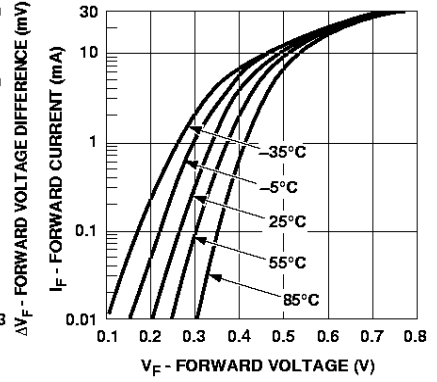
Figure 3. Typical Forward Current vs. Forward Voltage at Temperatures—HSMS-2810 Series.
