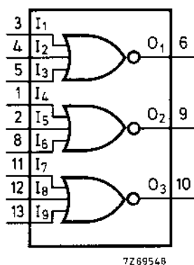
Fig.1 Functional diagram.
